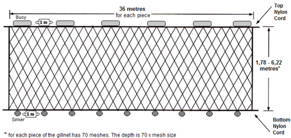
Figure 2. The illustration of the gillnet used in sampling.
